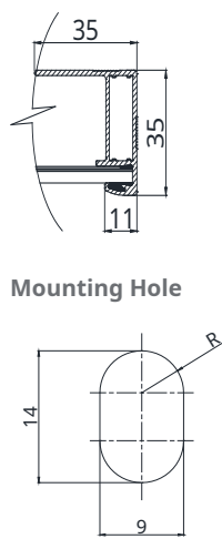
Frame Cross Section A-A
