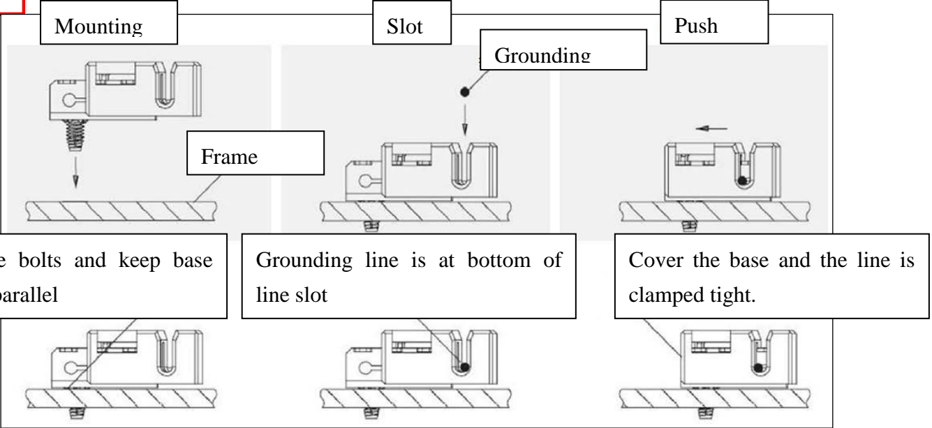
Figure 6 Grounding Clamp Installation
