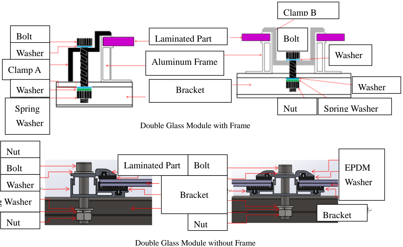
Figure 3 Clamp installation guideline
