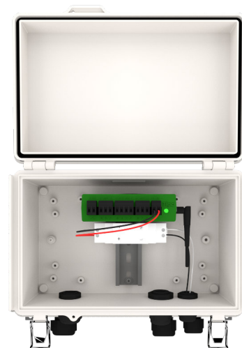
Pictured: CCA with DIN rail PSU in Outdoor Enclosure
